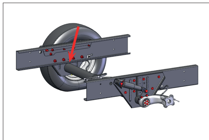
High frame chassis
