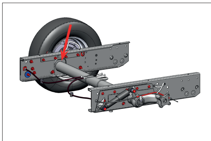
Low frame chassis
